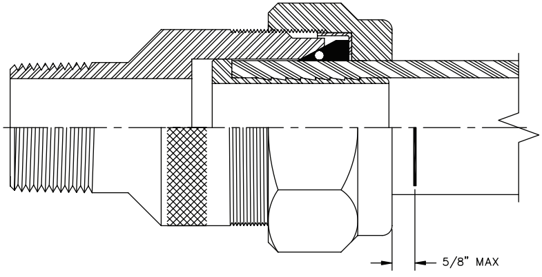
ORDER OF PARTS FOR 1 1/4" IPS PE COMPRESSION END
